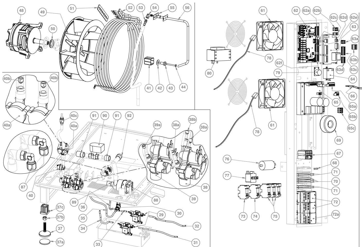
Exploded view 2/3
