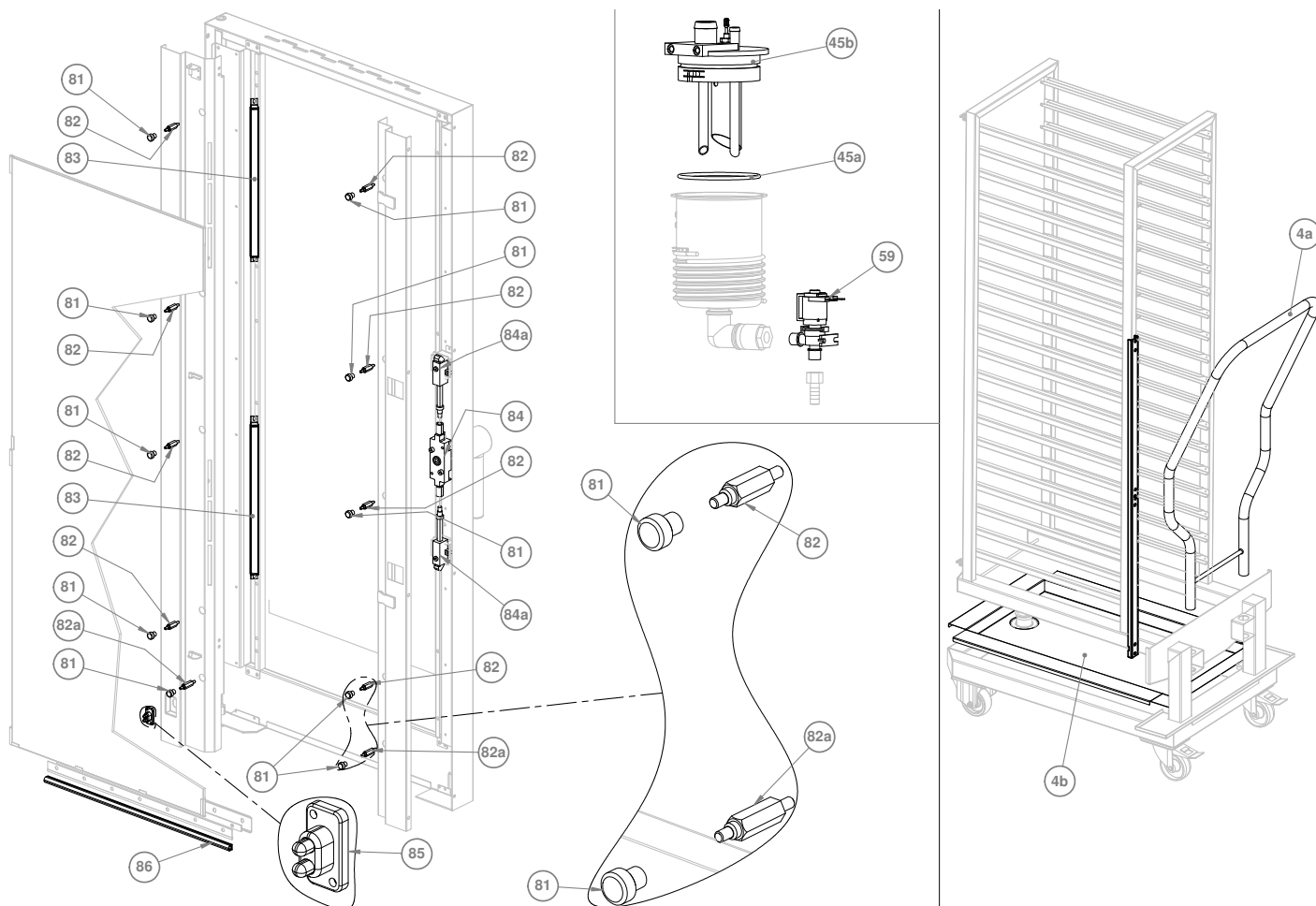
Exploded view 3/3
